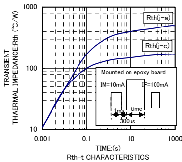
Rth-t CHARACTERISTICS
